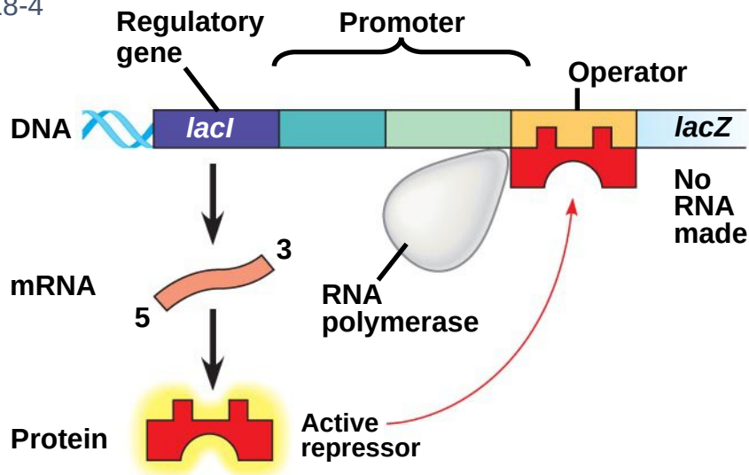
(a) Lactose absent, repressor active, operon off
